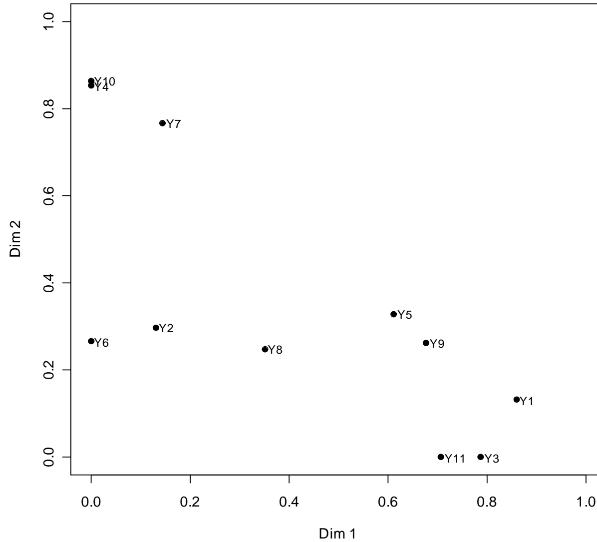
Weight representation
